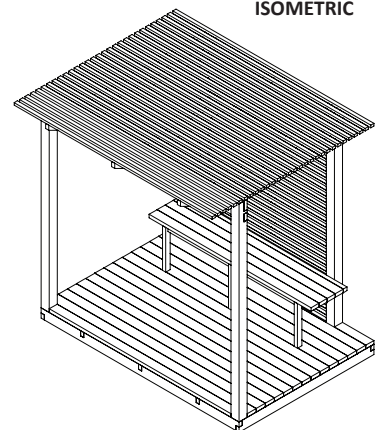
ISOMETRIC
