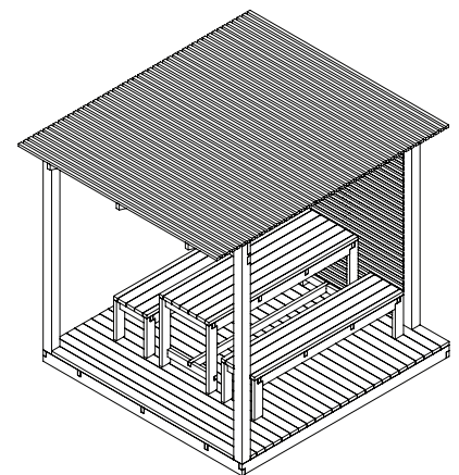
ISOMETRIC
